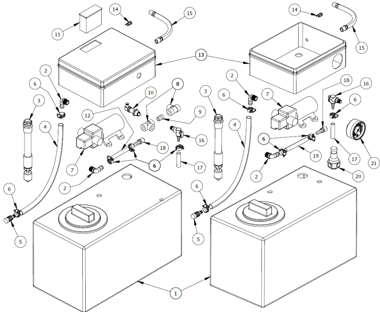
Glycol Feed with Digital Controller
