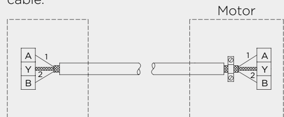
Fig. 3 Connection with screened 2-core cable.
