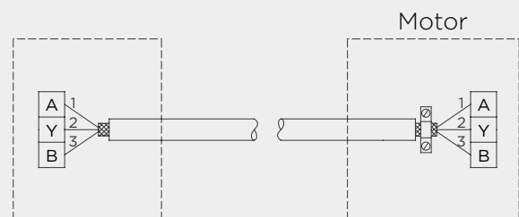
Fig. 2 Connection with screened 3-core cable.
